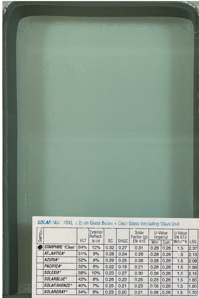
GL-1 INSULATING GLAZING UNIT
