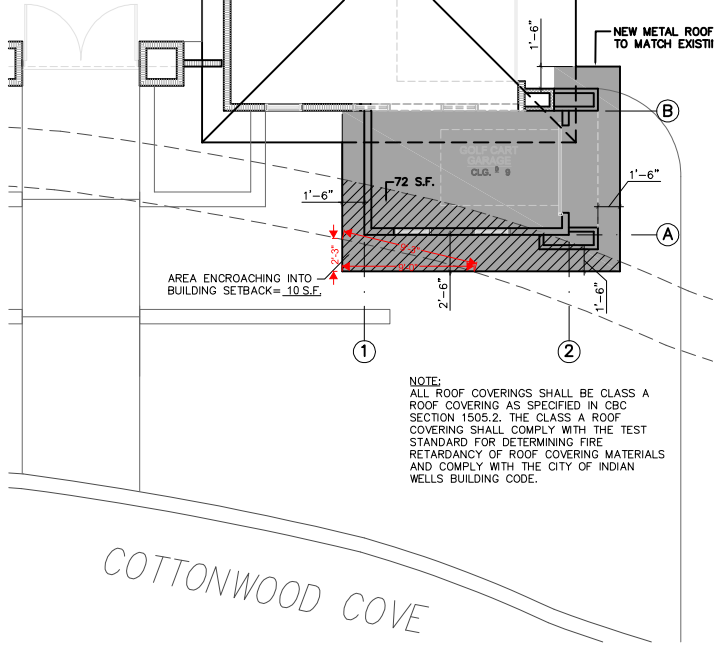
ROOF PLAN
