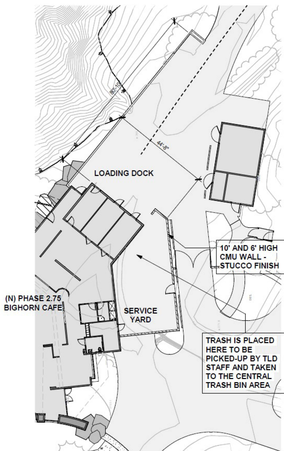
A LOADING DOCK PLAN 1" = 20'-0"
